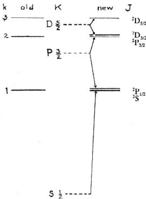
The old and the new term scheme of hydrogen [5]. The scheme shows the multiplet splitting of the excited states of the hydrogen atom with principal quantum number n=3 , presented by Goudsmit in the
