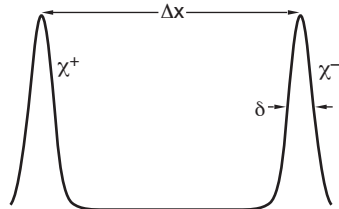
Figure 2. A “Schrödinger Cat” State or a Coherent Superposition This cat state \varphi(x) , the coherent superposition of two Gaussian wave packets of Equation (18), could describe a particle in a superposition of locations inside a Stern-Gerlach apparatus (see Figure 1) or the state that develops in the course of a double-slit experiment. The phase between the two components has been chosen to be zero.
